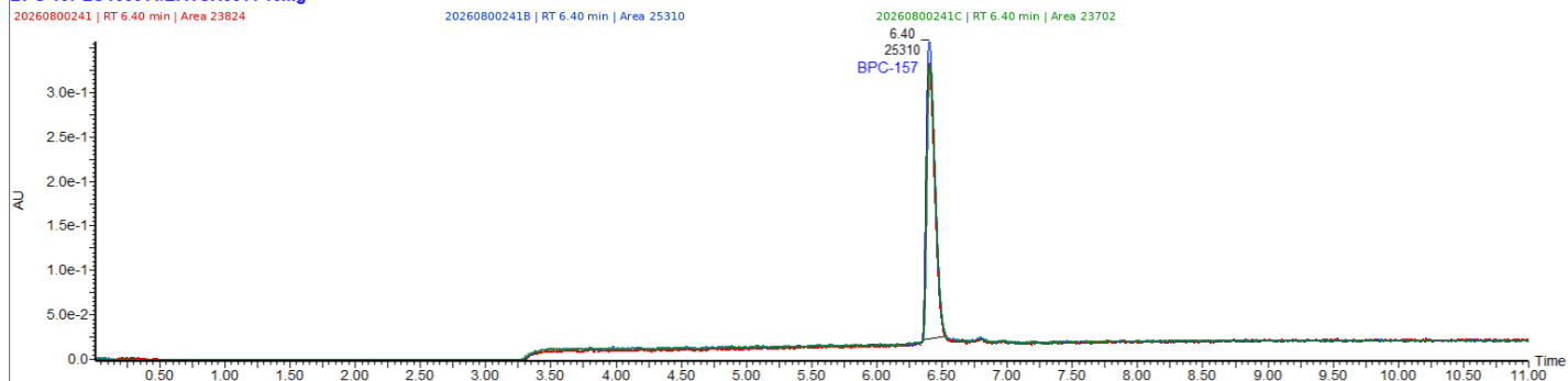
UV CHROMATOGRAM
