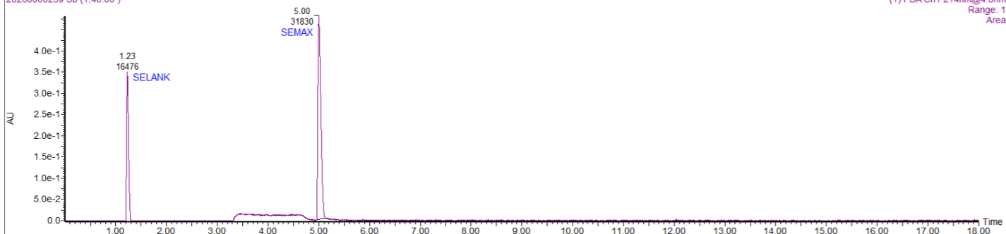
UV CHROMATOGRAM
