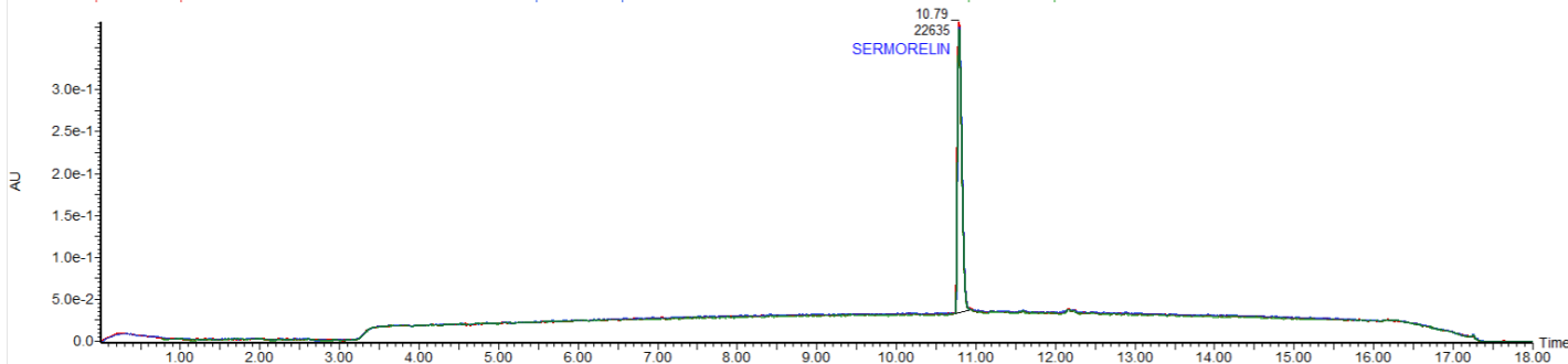
UV CHROMATOGRAM
