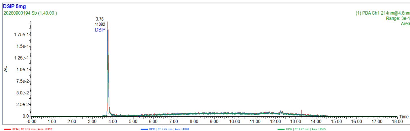
UV CHROMATOGRAM
