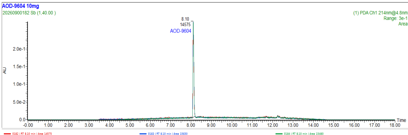
UV CHROMATOGRAM
